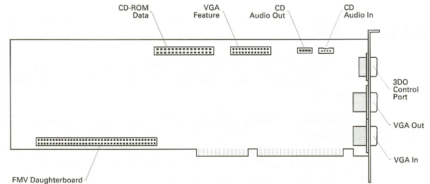
Figure 1-4: The connectors on your 3DO Blaster.
